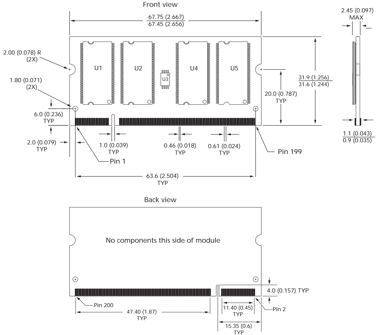
Figure 3: 200-Pin SODIMM
